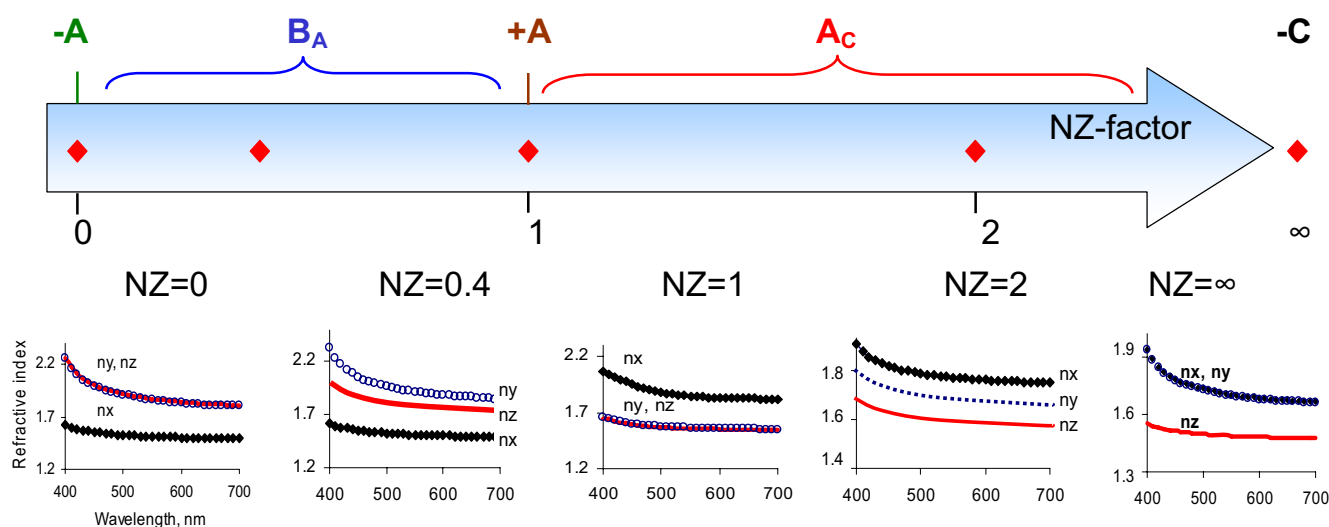
Fig. 1. Spectra of principal refractive indices for Crysoptix coatable retardation films: negative A-plate, biaxial B A -plate, positive A-plate, biaxial A C -plate, negative C-plate (shown from left to right).
